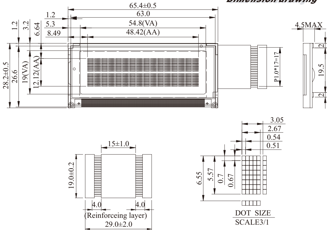
Dimension drawing
