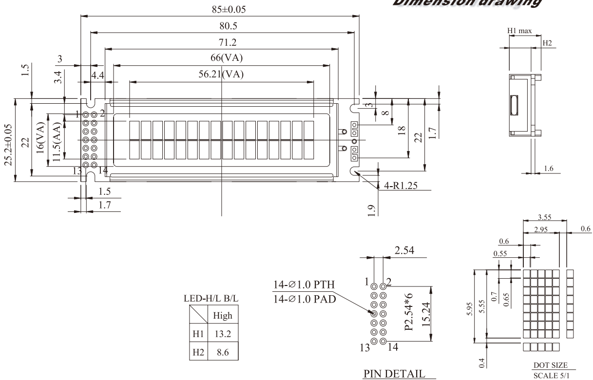
Dimension drawing
